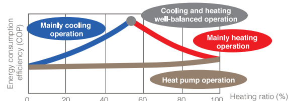
COP in the heat recovery system
